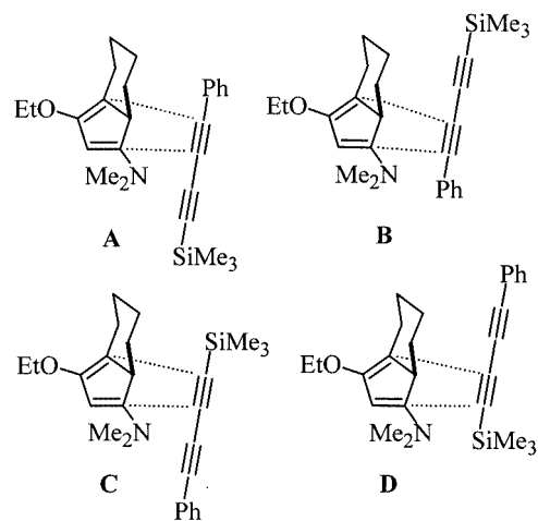
Figure 1. Four conceivable reaction modes of the intermediate cyclohexane-annulated (dimethylamino)ethoxycyclopentadiene 7 with phenyl(trimethylsilyl)butadiyne 2q
